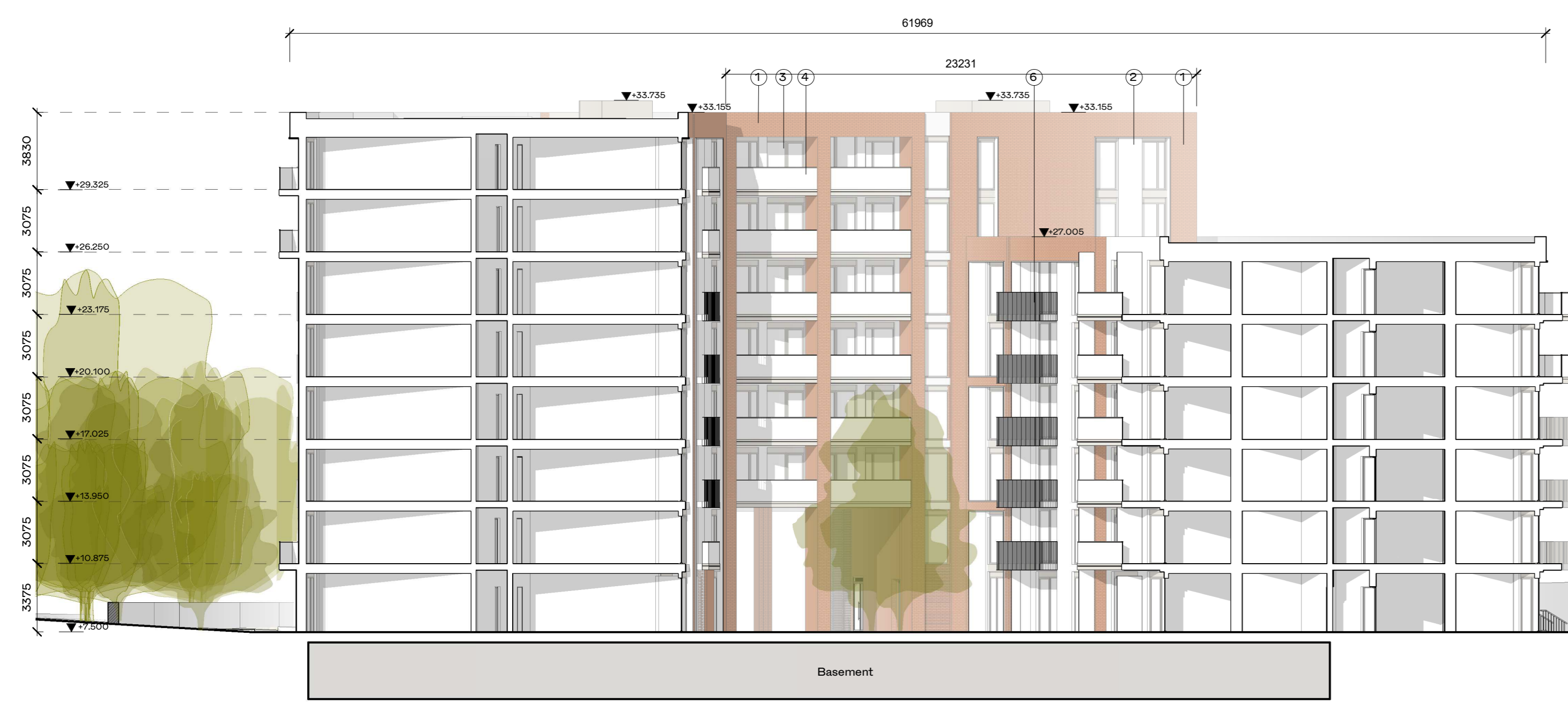
1 Block D2 Proposed South Courtyard Elevation 1: 200
